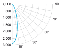
Narrow Flood 30° (3000K, 80 CRI)
