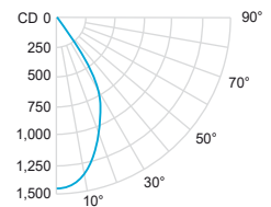
Wide Flood 58° (3000K, 80 CRI)
