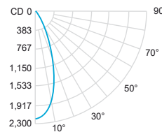
Flood 39° (3000K, 80 CRI)
